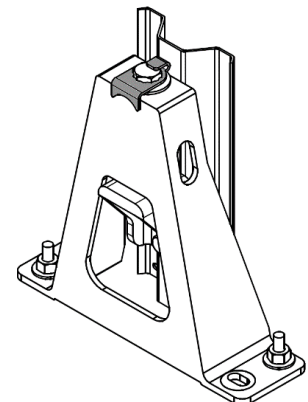
Figure 6b: Retention clip (shaded) over bolt.
