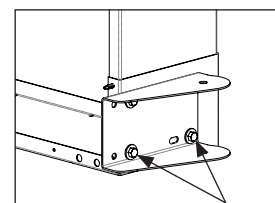
Offset mount for 2x6 mounting. Also applies to 819004 locking bracket.
